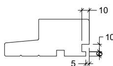
Bundkarmsnot type 6x10x10/5
