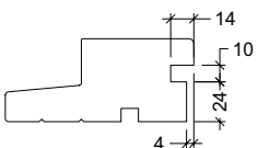
Bundkarmsnot type 24x10x14/4
