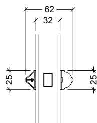
Classic alu 25mm energisprosse 2-lags rude
