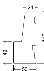
115mm karm
