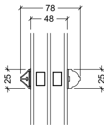
Classic alu 25mm energisprosse 3-lags rude
