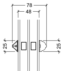
Classic alu 25mm energisprosse 3-lags rude
