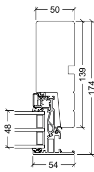
139mm karm
