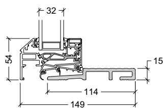
15mm HELO® bundkarm, terrasedør
