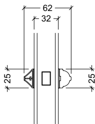
Classic alu 25mm energisprosse 2-lags rude
