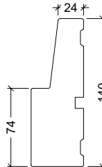
140mm karm
