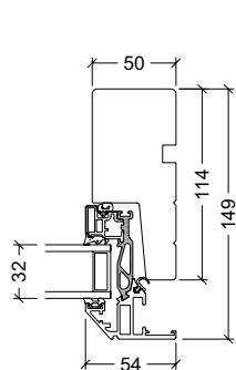
114mm karm
