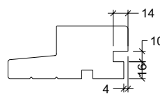
Bundkarmsnot type 16x10x14/4
